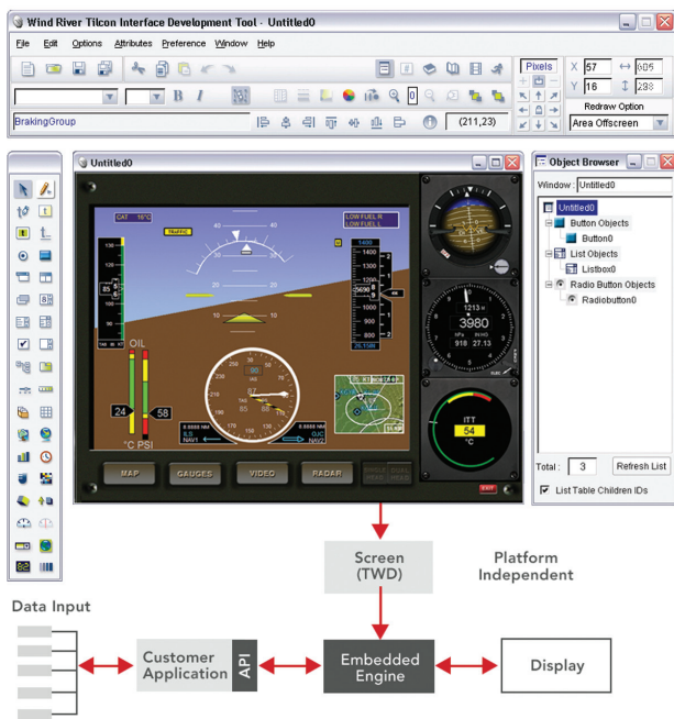
Figure 2: Wind River Tilcon Graphics Suite architecture
